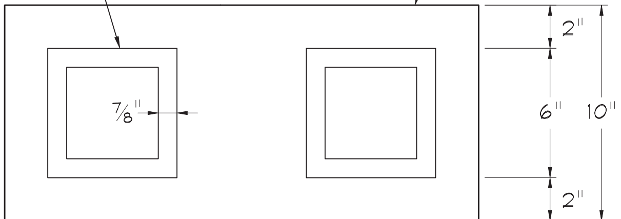
FRONT VIEW
